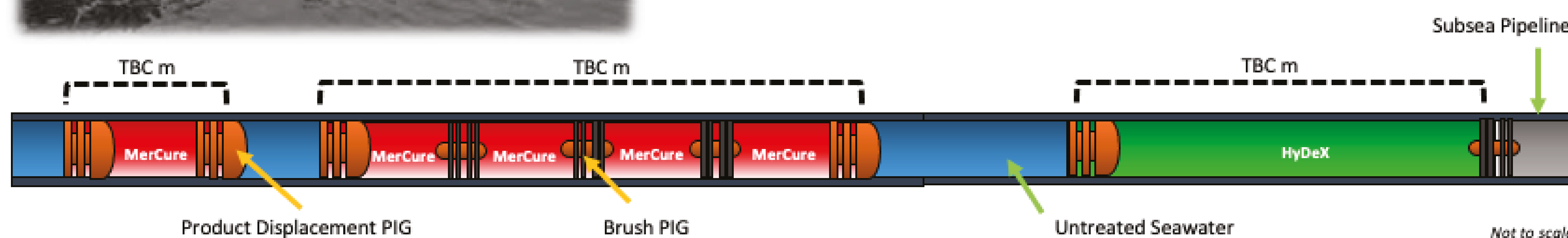
Example of In-situ pipeline decontamination using MerCure
